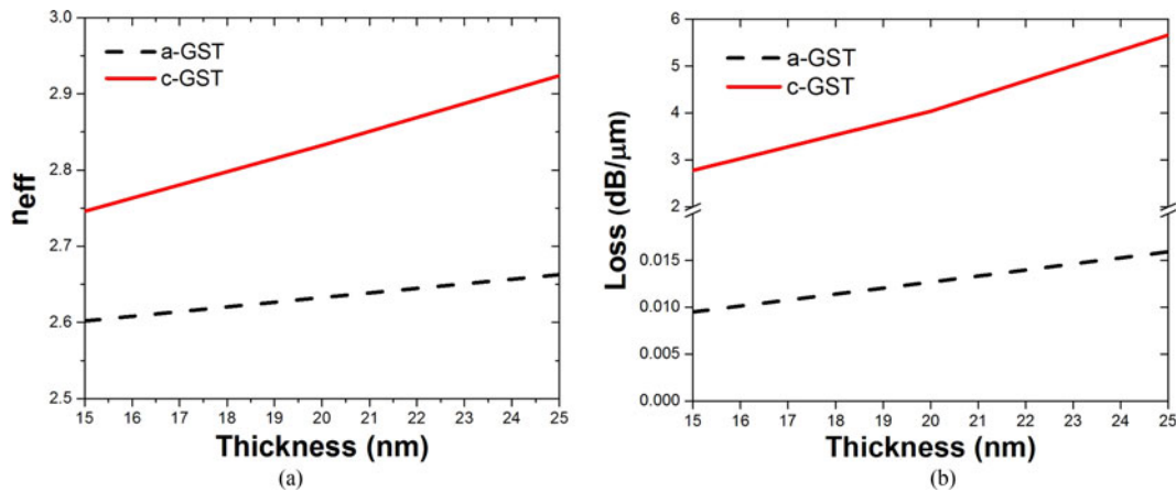
Fig. 7. VFEM simulation results showing the dependence of (a) the real part of the effective index and (b) and propagation loss of the Si-GST hybrid waveguide on the GST film thickness.
