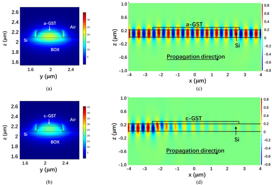
Fig. 3. (a), (b) Calculated modal profiles of the Si-GST hybrid waveguide along the cross-section AA' when the GST is in (a) the amorphous state and (b) the crystalline state. (c), (d) Electric field E_y component distribution along the propagation direction BB' when the GST is in (c) the amorphous state and (d) the crystalline state. The Si-GST hybrid waveguide length is 5 \mu\text{m} .
