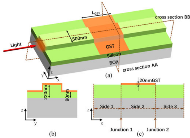
Fig. 2. (a) Schematic overview of the Si-GST hybrid waveguide. (b) Cross-sectional view along AA'. (c) Cross-sectional view along BB'.
