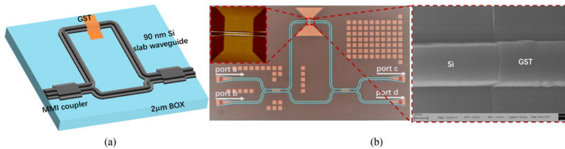
Fig. 4. (a) Schematic overview of the unbalanced Mach-Zehnder Interferometers. (b) Optical microscope image of the fabricated device. The left and right insets show the atomic force image (AFM) and scanning electron microscope (SEM) image of the Si-GST hybrid waveguide, respectively.
