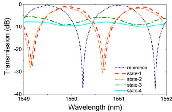
Fig. 5. Measured MZI transmission spectra when GST is at different states.
