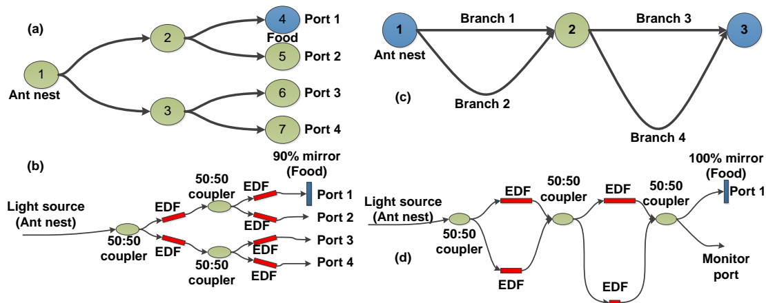
Fig. 1. Network design schemes used to demonstrate all-optical ACO: topology (a) and optical network realization (b) of a two-layer tree experiment; topology (c) and optical network realization (d) of a two-layer double bridge experiment.
