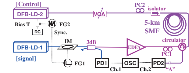
Fig. 2. Experimental setup. Distributed-feedback laser diode (DFB-LD); intensity modulator (IM); variable optical attenuator (VOA); polarization controller (PC); erbium-doped fiber amplifier (EDFA); single-mode optical fiber (SMF); function generator (FG); photo-diode (PD); oscilloscope (OSC).
