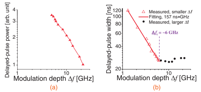
Fig. 5. Dependences of the power (a) and the width (b) of the delayed pulse on the linear modulation depth ( \Delta f ) of the cw control light. The dashed line in (b) corresponds to the critical modulation depth \Delta f_c \simeq 6 GHz.
